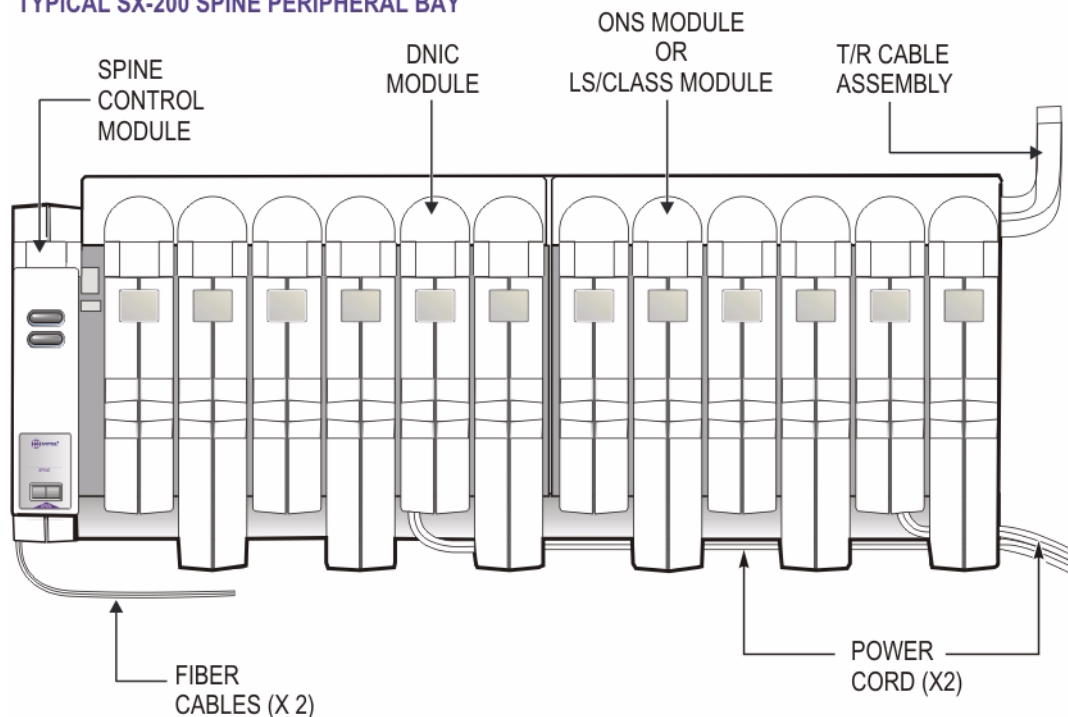
TYPICAL SX-200 SPINE PERIPHERAL BAY
